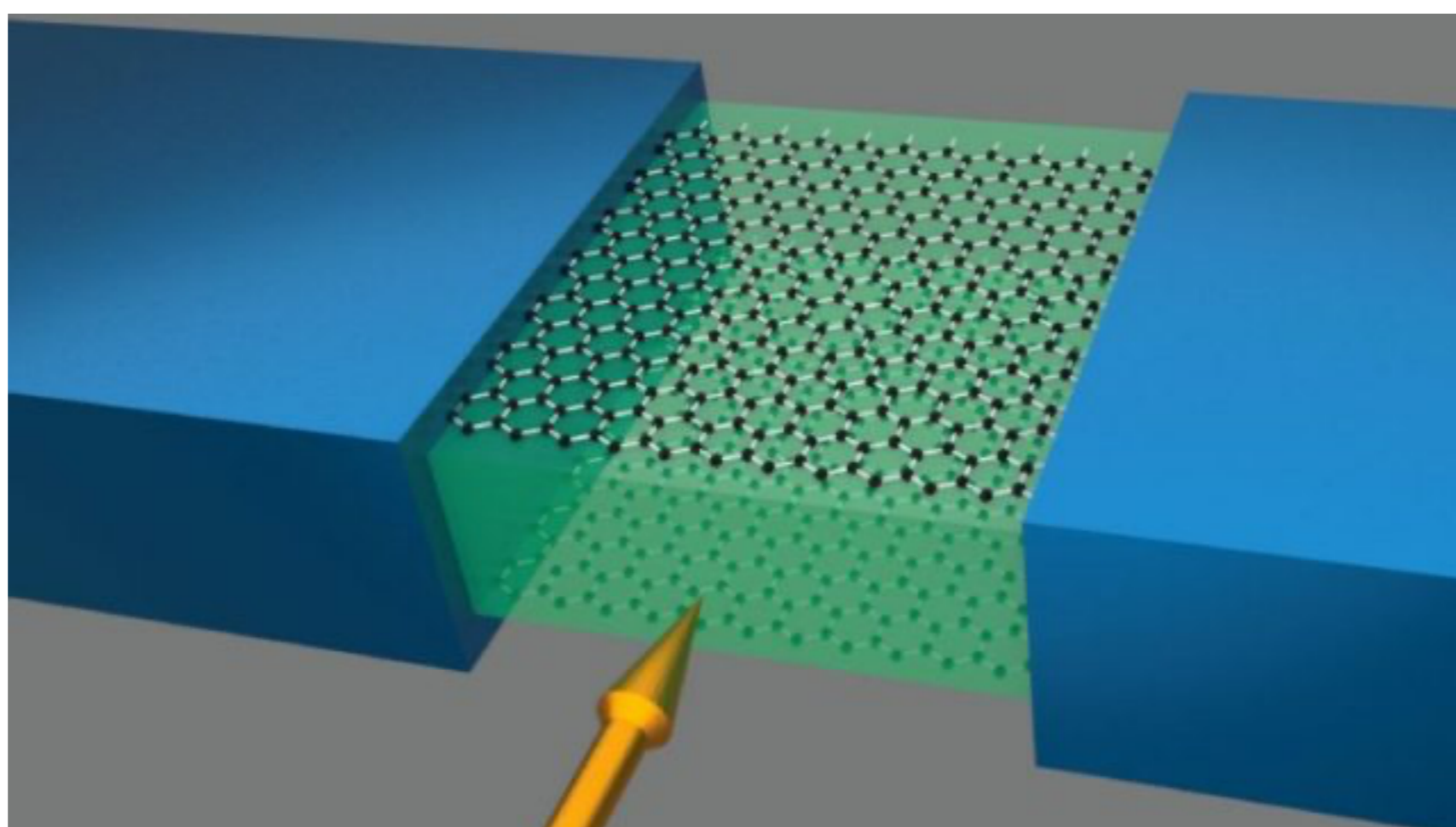
The new SQUID is made up of a stack of two-dimensional materials, including two graphene layers separated by a thin film of boron nitride. Credit: University of Basel, Department of Physics
