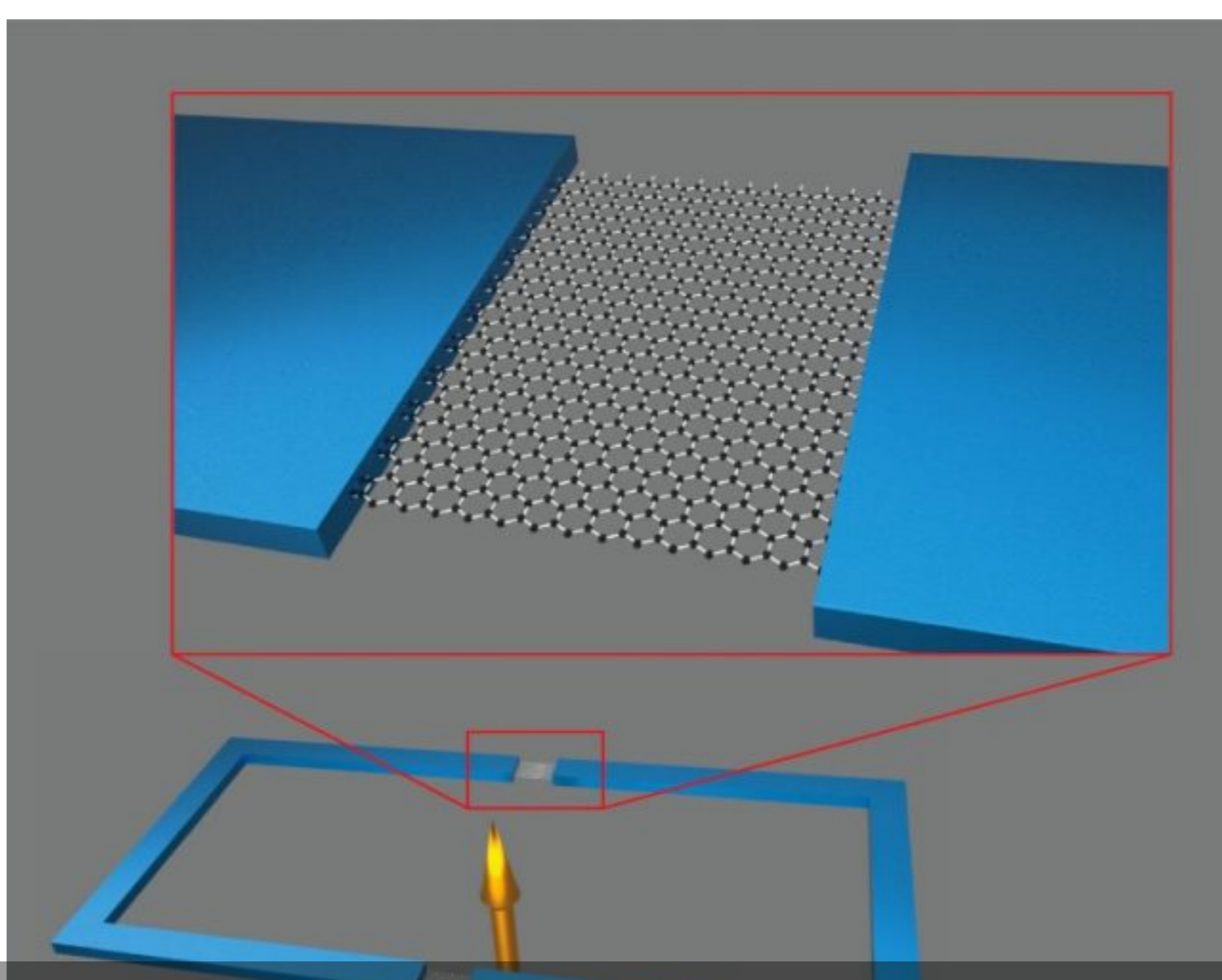
A conventional superconducting quantum interference device (SQUID) consists of a superconducting ring interrupted at two points by weak links (in this case a graphene layer). Credit: University of Basel, Department of Physics
